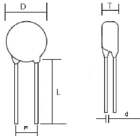
Straight leads (on request) Lead Style Code: 1
